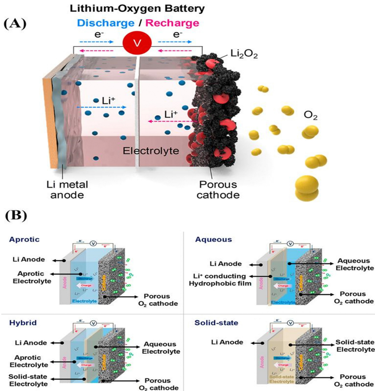
Fig. 9 (A) Schematic representation of a Li- \text{O}_2 battery. (B) Schematic configuration of all types of Li- \text{O}_2 cells. 145
