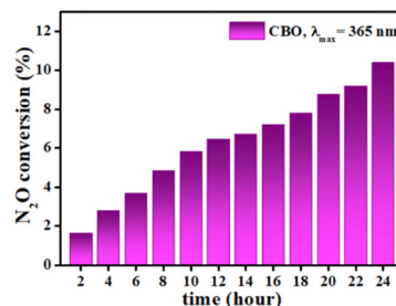
Fig. 6 Time dependence on the \text{N}_2\text{O} conversion during the photocatalytic decomposition of \text{N}_2\text{O} over CBO under UV-A irradiation at 365 nm.
