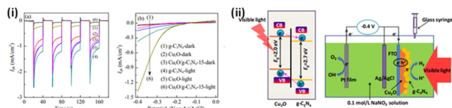
Fig. 8 (i) (a) Transient photocurrent response at a bias potential of -0.4\text{ V} (vs. Ag/AgCl) under visible light: [(1) Cu_2O ; (2) Cu_2O/g-C_3N_4-5 ; (3) Cu_2O/g-C_3N_4-10 ; (4) Cu_2O/g-C_3N_4-15 ; (5) Cu_2O/g-C_3N_4-20 ; (6) g-C_3N_4 ]. (b) Linear sweep voltammograms of Cu_2O , g-C_3N_4 and Cu_2O/g-C_3N_4-15 films in the dark and under visible light. (ii) Schematic pathway for photoelectron transfer and the photoelectrochemical process in Cu_2O/g-C_3N_4 film under visible light irradiation. Reprinted from ref. 151 with permission.
