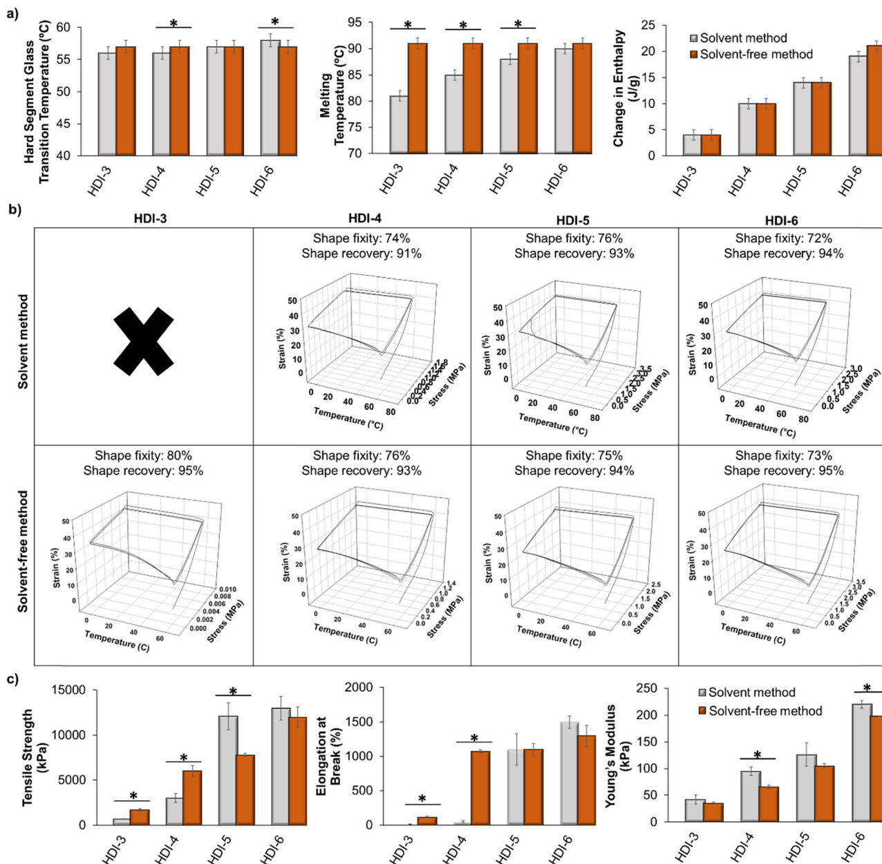
Fig. 3 Comparison of (a) thermal ( n = 3 ), (b) shape memory ( n = 1 , ✗: no shape memory properties were observed), and (c) tensile ( n = 3 ) properties of polymers synthesized using solvent-based (data are from our previous work 32 ) and solvent-free methods. Mean \pm standard deviation displayed. * p < 0.05 relative to corollary sample synthesized using solvent-based method.
