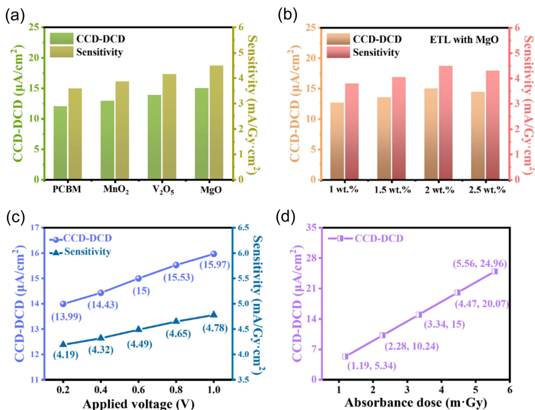
Fig. 12 (a) CCD-DDC and sensitivity variations in the X-ray detectors with the pure and \text{V}_2\text{O}_5 , \text{MnO}_2 , and \text{MgO} blended PCBM ETL; (b) CCD-DDC and sensitivity at different concentrations (1, 1.5, 2 and 2.5 wt%) of \text{MgO} blended PCBM ETL; (c) CCD-DDC and sensitivity at different applied bias voltages of the \text{MgO} blended PCBM ETL using a fabricated X-ray detector; (d) CCD-DDC at different dose rate outcomes of the \text{MgO} blended PCBM ETL using a fabricated X-ray detector.
