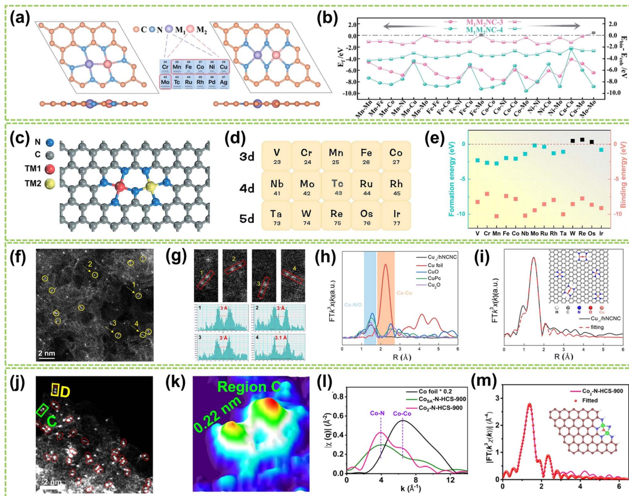
Fig. 3 Structure characterization of homonuclear DACs connected by heteroatomic bridges. (a) The top and side views of optimized M_1M_2NC-3 and M_1M_2NC-4 . (b) E_i and differences between the binding and cohesive energies of DACs ( \Delta E_{b-c} ) 37 (reproduced with permission from ref. 37 copyright 2022, RSC). (c) Structure of N-bridged M_1-N-M_2/NC . (d) 14 transition metals are taken into account in this work. (e) E_i and E_b of M_1-N-M_2/NC 38 (reproduced with permission from ref. 38 copyright 2023, Springer Nature). (f) HAADF-STEM image showing twinned Cu atoms (circled) and isolated Cu atoms. (g) Corresponding enlargement of the sites 1–4 in (f) and intensity profiles. (h) FT-EXAFS spectra of Cu_{-1}/hNCNC and the references. (i) FT-EXAFS fitting curve of the Cu K-edge in R-space for Cu_{-1}/hNCNC and the corresponding structure diagram 39 (reproduced with permission from ref. 39 copyright 2024, ACS). (j) AC HAADF-STEM images (Co dual atoms marked by red circles). (k) 3D atom-overlapping Gaussian-function fitting map in (j) for Co_2-N-HCS-900 . (l) q -Space magnitude comparisons of Co foil, Co_{SA}-N-HCS-900 , and Co_2-N-HCS-900 . (m) k^3 -Weighted EXAFS fitting curves at R space for Co_2-N-HCS-900 (inset: schematic structure of Co_2N_5 models; green: Co, blue: N, red: O) 40 (reproduced with permission from ref. 40 copyright 2023, Springer Nature).
