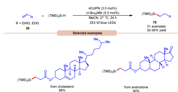
Scheme 30 Bromine radical-mediated hydrosilylation of alkenes using (TMS)_3SiH .
