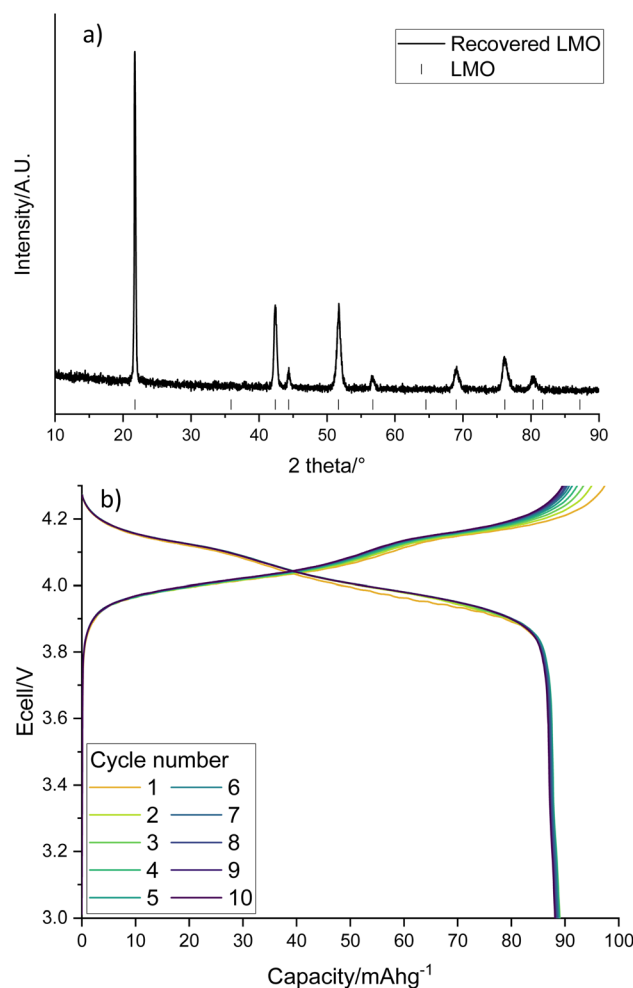
Fig. 6 (a) XRD pattern of recovered LMO (Co Kα) with tick marks correspond to LMO and (b) galvanostatic charge–discharge profile of recovered LMO when cycled at 10 mAg -1 between 3–4.3 V.
