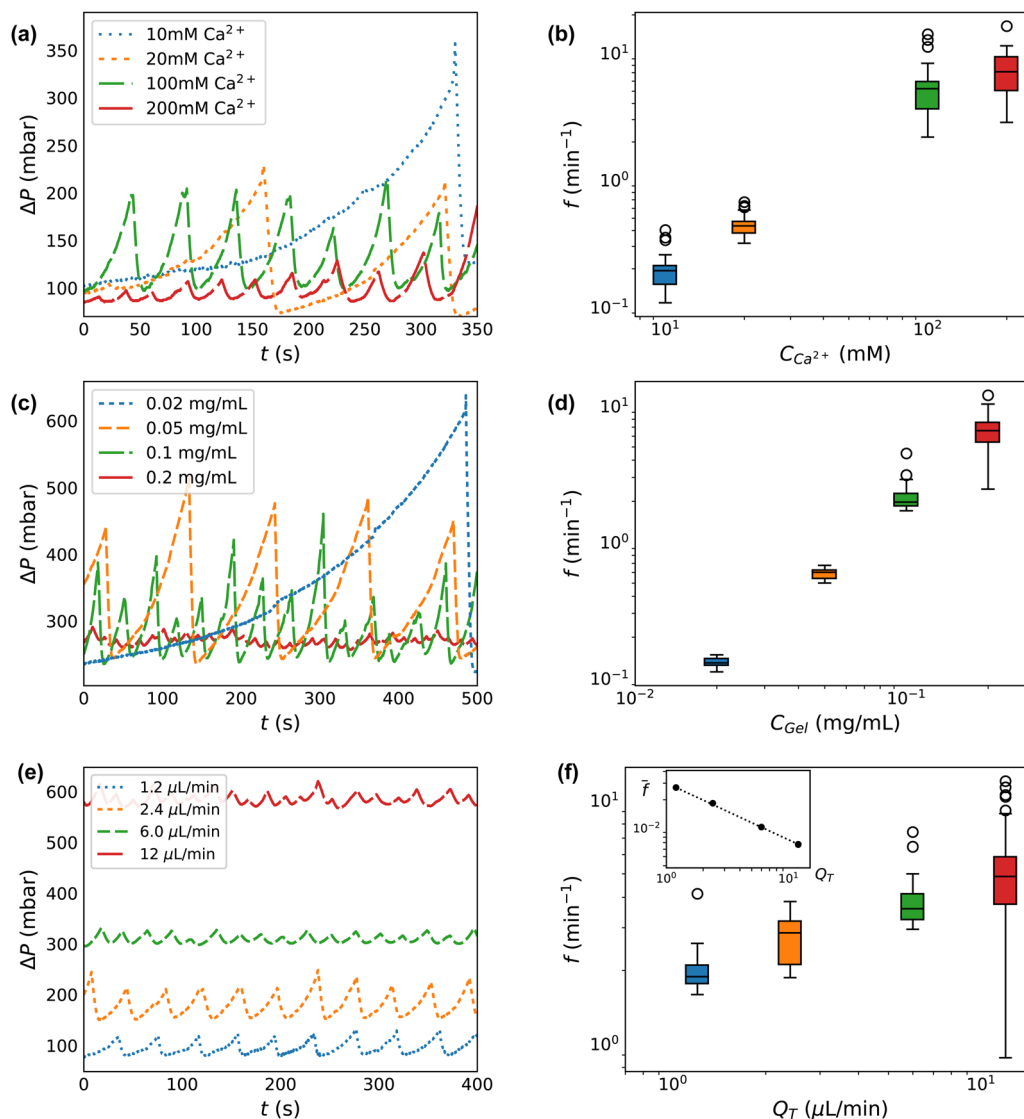
Fig. 3 Clog size and frequency of ablation is controllable with system parameters. (a), (c) and (e) Select raw pressure traces from experiments varying calcium C_{\text{Ca}^{2+}} , total concentration C_{\text{Gel}} , and total flow rate Q_T respectively. (b), (d) and (f) Frequency histogram of peak pressures for experiments varying C_{\text{Ca}^{2+}} , C_{\text{Gel}} , and Q_T , and respectively. The inset in (f) is the frequency normalized by the baseline shear rate which demonstrates that clogs form less frequently when accounting for flow rate. The box and whisker plots show the median value of a group as horizontal lines. The boxes encompass the first to the third quartile. The whiskers extend 1.5 times the interquartile range. The experimental conditions for each plot correspond to those shown in Table 1.
