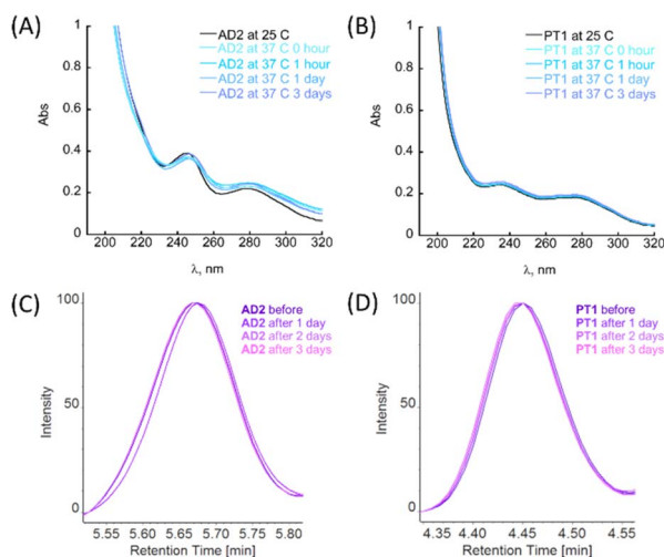
Fig. 4 Stability of (A) AD2 and (B) PT1 under physiological conditions (pH = 7.4 and T 37 °C), as monitored by UV-Vis. Conditions: [ PT1 ] = [ AD2 ] = 100 μM, [PBS] = 50 mM. Proteolysis experiments: overlap of the retention peaks of (C) AD2 and (D) PT1 from the corresponding HPLC chromatograms ( \lambda = 214 nm, a linear gradient of 5–95% ACN/ H_2O 0.1% TFA over 10 min, at a flow rate of 0.7 min mL -1 on the analytical C18 column), taken at different times from the proteolytic stability experiment. Conditions: [ PT1 ] = [ AD2 ] = 0.1 mg mL -1 , [trypsin] = 0.1 μM, [PBS] = 50 mM (pH = 7.4), at the constant temperature of 37 °C.
