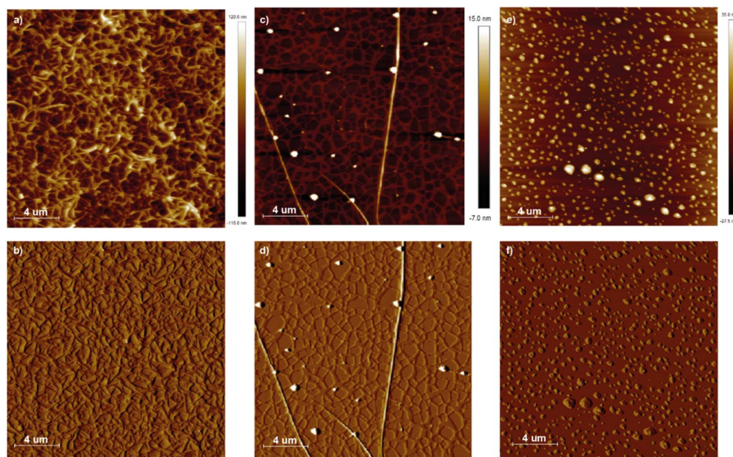
Fig. 4 Height (a, c and e) and phase (b, d and f) AFM images of NPDIs 2 (a, b, MCH, 100 \mu\text{M} ); 3 (c, d, MCH, 150 \mu\text{M} ) and 4 (e, f, MCH, 250 \mu\text{M} ) onto HOPG as surface.
