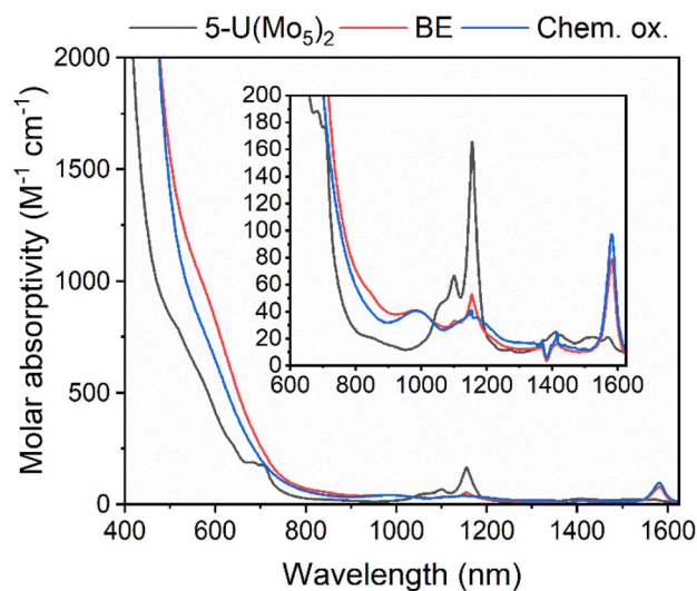
Fig. 9 UV-vis/NIR spectra of pristine 5\text{-U}(\text{Mo}_5)_2 (black), after bulk electrolysis of 5\text{-U}(\text{Mo}_5)_2 at 0.78 V vs. Fc/Fc^+ (red, BE), and after treatment of 5\text{-U}(\text{Mo}_5)_2 with an excess of [\text{NO}][\text{PF}_6] (blue, Chem. ox.). The region between 600 and 1600 nm is expanded to highlight the f-f transitions. All spectra were recorded in DCM.
