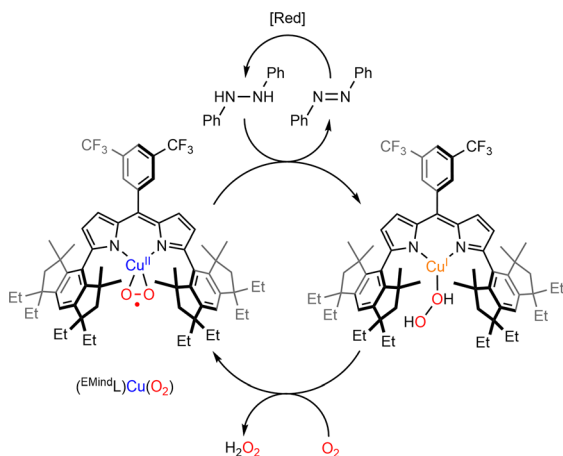
Scheme 7 Reaction of [(^{\text{E}}\text{MindL})\text{Cu}^{\text{II}}(\text{O}_2)] with 1,2-diphenylhydrazine to produce azoarene and [(^{\text{E}}\text{MindL})\text{Cu}^{\text{I}}(\text{H}_2\text{O}_2)] . Adapted from ref. 83.
