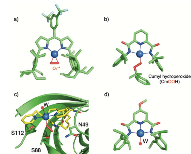
Fig. 6 Selected crystallographic structures of recently described mononuclear copper–oxygen adducts. a) \eta^2 -superoxo based on the ^E\text{M}^{\text{ind}}\text{L} ligand. 83 Hydrogen atoms were omitted for clarity; b) The anion [(L)Cu(OOCm)] - based on the bis(arylcarboxamido)-pyridine ligand. 85 Hydrogen atoms and the Et 4 N + counter ion were omitted for clarity; c) \eta^1 -Hydroperoxido complex in an artificial enzyme based on a streptavidin scaffold: [(biot-et-dpea)Cu II (OOH)(OH 2 )] + c Sav; 86 d) High-valent [(L)CuOH] species based on the bis(arylcarboxamido)-pyridine ligand (W as deprotonated water ligand). 87
