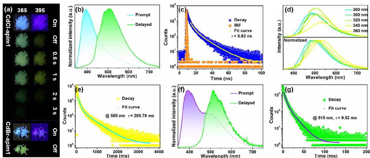
Fig. 3 (a) Photographs of \text{CdCl}_2\cdot\text{apim}_1 and \text{CdBr}_2\cdot\text{apim}_1 before and after removing the 365/395 nm UV lamp; the prompt and delayed spectra of \text{CdCl}_2\cdot\text{apim}_1 (b) and \text{CdBr}_2\cdot\text{apim}_1 (f); (c) fluorescence decay profile of \text{CdCl}_2\cdot\text{apim}_1 ; (d) delayed spectra of \text{CdCl}_2\cdot\text{apim}_1 excited by different wavelengths; phosphorescence decay profiles of \text{CdCl}_2\cdot\text{apim}_1 (e) and \text{CdBr}_2\cdot\text{apim}_1 (g).
