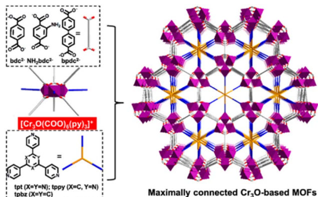
Fig. 13 The structural components, together with the framework viewed along the c axis. \text{NH}_2\text{bdc}^{2-} = 2-aminoterephthalate, \text{bpd}c^{2-} = biphenyl-4,4'-dicarboxylate, \text{tpt} = 2,4,6-tri(4-pyridyl)-1,3,5-triazine ( \text{tpt} ) into the pores, the moisture stability of the MOFs with \text{tpt} substitution rose dramatically. Recently, Bu and colleagues prepared a family of acid/base-resistant Cr-MOFs by dividing the large pore of the original Cr-MOFs into interconnected small pores employing triangle ligands (Fig. 13). 153 The newly formed Cr-MOFs (CPM-243(F)) could maintain their crystallinity even under very severe conditions such as HCl aqueous solution and 10 M NaOH aqueous solution. Such exceptional stability was due to the presence of the multi-binding pore-partitioning ligand, framework rigidity, and highly connected \text{Cr}_3\text{O} nodes.
