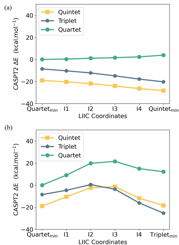
Fig. 8 CASPT2 computed potential energy surface using an (ne, 18o) active space along the linear interpolation of internal coordinates (LIIC) between the PBE0 optimized (a) \text{U}^{\text{Me6}} high spin ( S = 3/2 ) and [\text{U}^{\text{Me6}}]^- high spin ( S = 2 ) geometries and (b) \text{U}^{\text{Me6}} high spin ( S = 3/2 ) and [\text{U}^{\text{Me6}}]^- intermediate spin ( S = 1 ) geometries. Note that the S = 2 state on its DFT-optimised structure, right most point in (a), is the lowest energy point in either plot.
