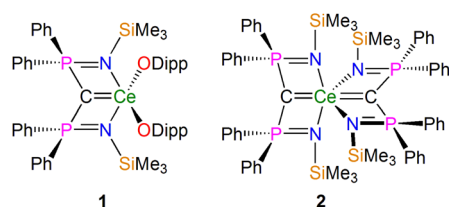
Fig. 2 Cerium-carbene complexes 1 and 2 . These complexes are the two subject molecules of this study. Dipp = diisopropylphenyl.
