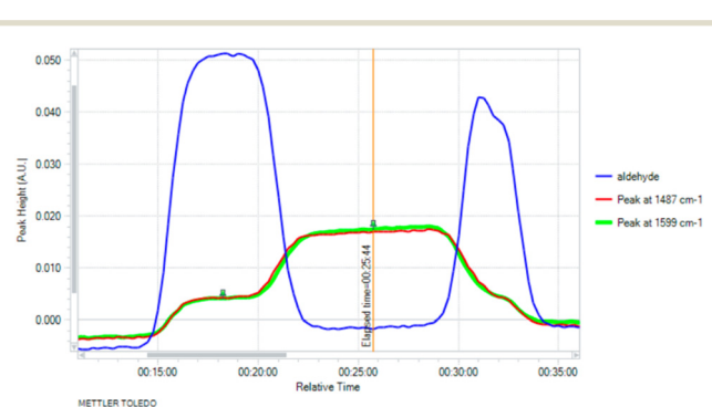
Fig. 2 Consumption of aldehyde starting material when hydrazine reagent is injected, and identification of peaks at 1487 \text{cm}^{-1} and 1599 \text{cm}^{-1} indicative of the presence of the intermediate.
