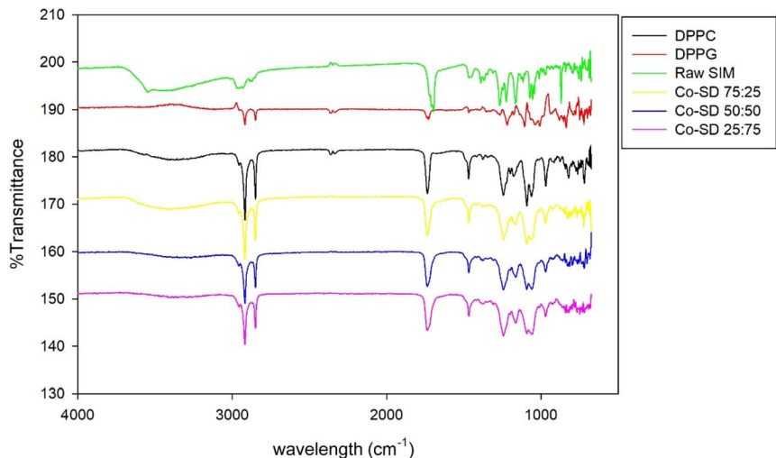
Fig. 5 ATR-FTIR spectra of raw Sim, DPPC, DPPG, Co-SD Sim : PL 25 : 75, Co-SD Sim : PL 50 : 50, and Co-SD Sim : PL 75 : 25 powders where PL is DPPC/DPPG.
