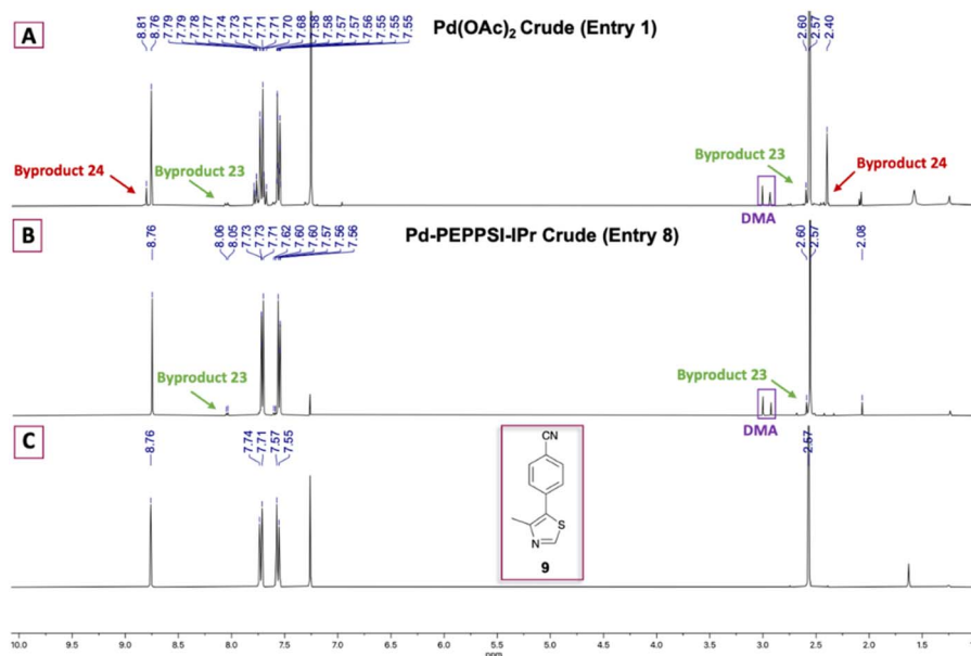
Fig. 1 ^1\text{H} NMR comparison of crude 9 formed using (A) 0.1 mol% \text{Pd}(\text{OAc})_2 and (B) 0.5 mol% \text{Pd} -PEPPSI-IPr. (C) ^1\text{H} NMR spectrum of purified 9 .
