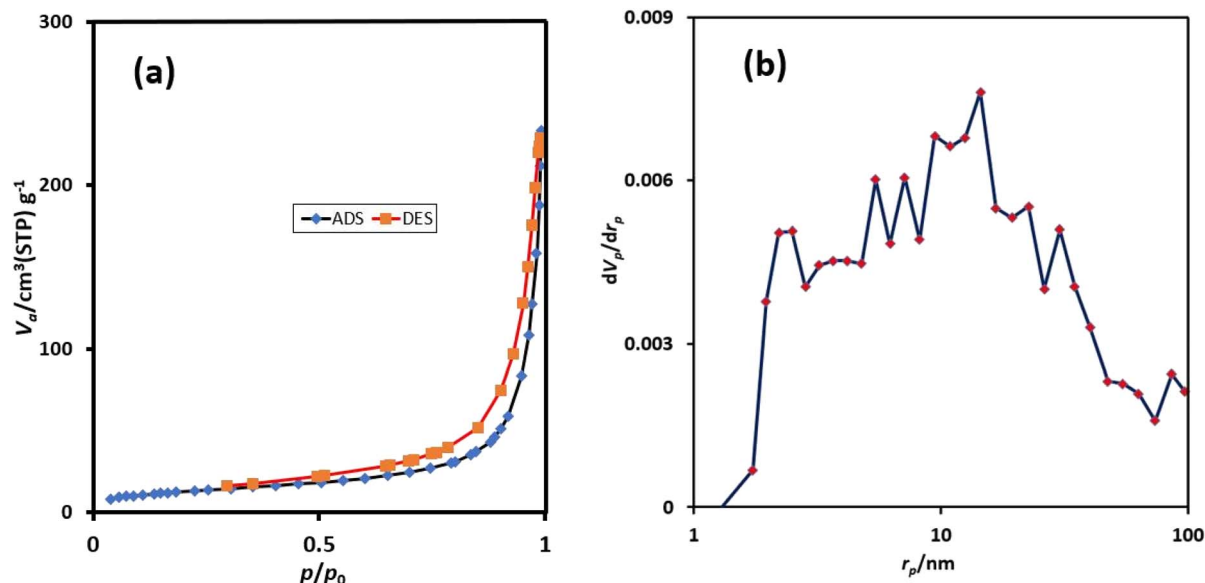
Fig. 4 The N_2 adsorption-desorption isotherms of urea-rich POP (a) and pore size distribution curves of urea-rich POP (b).
