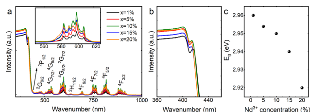
Fig. 6 Diffuse reflectance spectra of the \text{CsPbCl}_3 : x\% \text{Nd}^{3+} perovskite powders (a) together with an enlarged spectrum showing the exciton band (b) and energy gap values as a function of dopant concentration (c).
