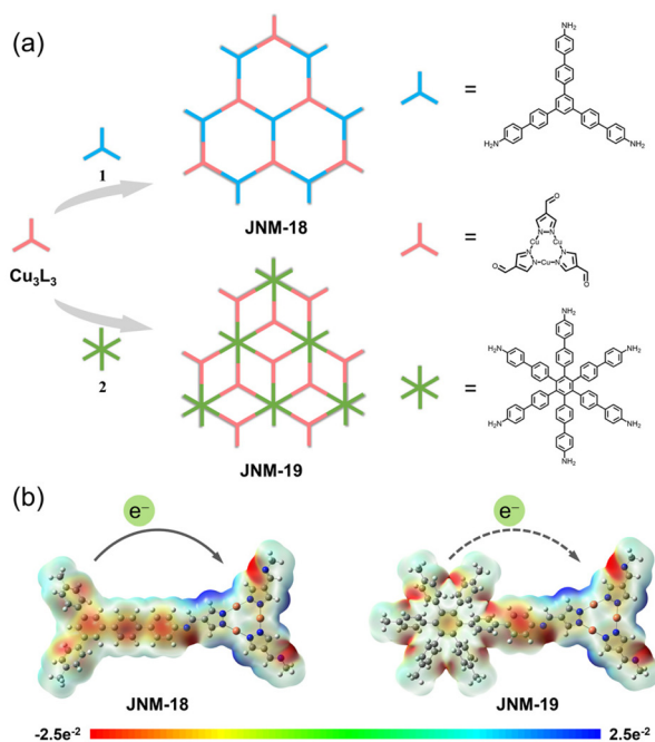
Fig. 1 (a) Syntheses of imine-linked D-A MOFs, JNM-18 and JNM-19 , via Schiff base reactions between the Cu 3 CTU acceptor ( \text{Cu}_3\text{L}_3 ) and TPB ( 1 ) or HPB ( 2 ) donors, respectively. (b) The ESP surface maps for the optimized structures of JNM-18 (left) and JNM-19 (right). The planar TPB moiety in JNM-18 shows a stronger electron donating ability than the HPB unit with nonplanar propeller arrangement in JNM-19 .
