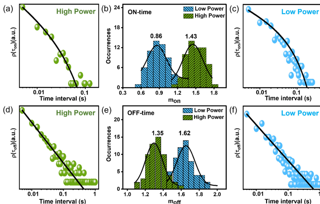
Fig. 4 (a and c) The probability distribution plots of ON time durations of a QD at low ( \sim 2 W cm -2 , c) and high ( \sim 20 W cm -2 , a) excitation powers. (d and f) Similar plots for OFF time durations at low ( \sim 2 W cm -2 , f) and high ( \sim 20 W cm -2 , d) excitation powers. (b) Probability histograms of the ON time power law exponents ( m_{\text{on}} ) recorded over 60–70 particles at low and high powers. (e) Same plots for m_{\text{off}} at two different powers. The mean values are mentioned above each distribution. As the pump intensity increases relative charge trapping rate ( m_{\text{on}} ) rate increases (b), whereas the relative charge de-trapping rate ( m_{\text{off}} ) decreases (e), implying more efficient charge trapping at high power.
