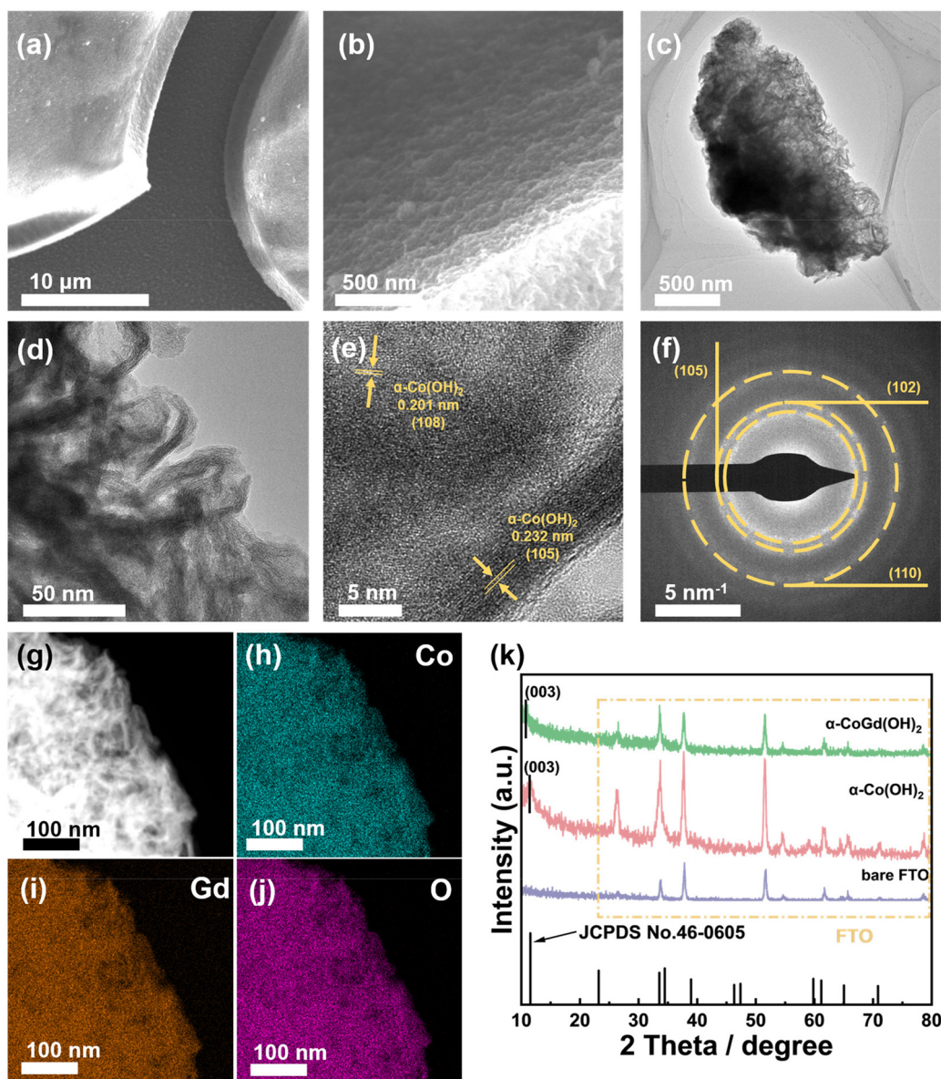
Fig. 2 (a and b) The FESEM images of \alpha -CoGd(OH) _2 /FTO. (c and d) The TEM images, (e) HRTEM image, and (f) SAED pattern together with the corresponding (g) HAADF pattern as well as the elemental mapping of (h) Co, (i) Gd, and (j) O for \alpha -CoGd(OH) _2 peeled from the FTO substrate. (k) The powder XRD patterns of bare FTO, \alpha -Co(OH) _2 /FTO, and \alpha -CoGd(OH) _2 /FTO.
