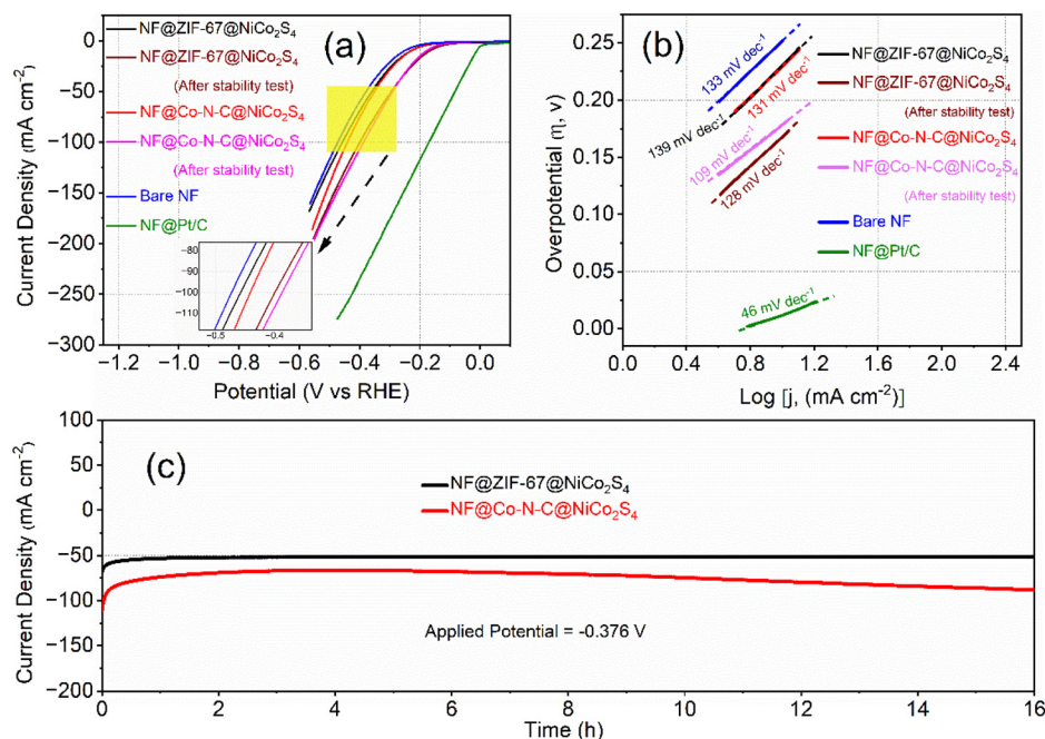
Fig. 6 HER analysis: (a) LSV curves recorded at a scan rate of 2 mV s -1 ( i R corrected), (b) Tafel curves and (c) CA curves.
