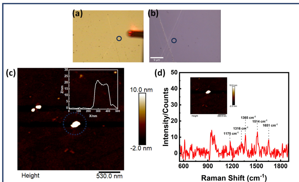
Fig. 5 Single molecule SERS measurements of the EGFR protein immobilized in the Au NR dimer nanoantenna system, (a and b) optical images recorded using an AFM (10× objective) and confocal Raman microscope (100× objective), respectively, (c) AFM images of Au NR dimer with the corresponding height profile in the inset and (d) the corresponding SERS spectrum of an EGFR molecule with the AFM image of a single nanoantenna in presented inset. (Strategy I) The blue dotted circle represents the dimer structure probed for analysis.
