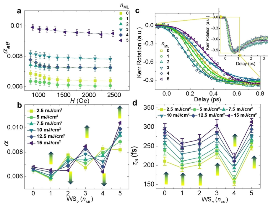
Fig. 3 (a) Dependence of the effective damping parameter \alpha_{eff} on the magnetic field H for WS_2 ( n_{ML} )/ Co_3FeB at a fixed pump fluence ( 10 \text{ mJ cm}^{-2} ). Dotted lines correspond to fits to exponentially decaying functions. (b) Variation of \alpha with n_{ML} at various pump fluences ( 2.5\text{--}15 \text{ mJ cm}^{-2} ) at an external bias field of 1.56 \text{ kOe} . Coloured arrows indicate the increment of fluence. (c) Ultrafast demagnetization curves of WS_2 ( n_{ML} )/ Co_3FeB . The inset shows the time-resolved Kerr rotation over a longer time scale. Solid lines are fits to eqn (1). (d) Variation of \tau_m with n_{ML} at different pump fluences ( 2.5\text{--}15 \text{ mJ cm}^{-2} ). Coloured arrows indicate the increment of fluence.
