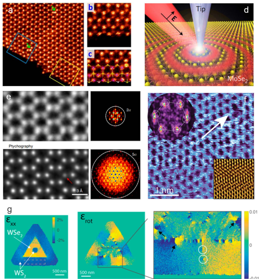
Fig. 3 Mosaic of the experimental data from the state of metrology for 2D materials reported in this review. (a–c) Intrinsic point defects in monolayer MoSe 2 by STEM-ADF. (d) Schematic of nano-optical imaging study of waveguide MoSe 2 using tip-enhanced SPM methods. (e) An electron microscope and pixel-array detector are used to record the complete distribution of transmitted electrons and full-field ptychography in MoS 2 . (f) Contact-mode electrical AFM is used to map barrier inhomogeneities in WS 2 . (g) Strain mapping at the WS 2 –WS 2 junction using an electron microscope pixel array detector (EMPAD) in TEM. Panels adapted with permission as follows: panel (a–c); 22 panel (d); 75 panel (e); 76 panel (f); 31 panel (g). 26
