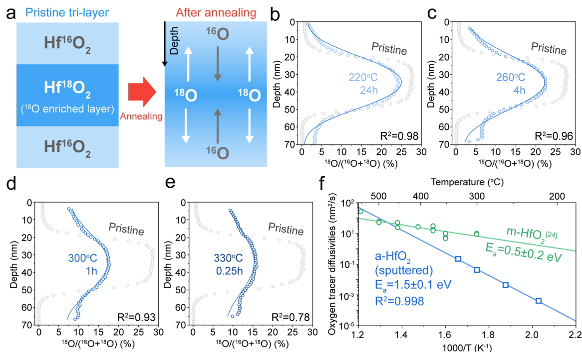
Fig. 2 Oxygen tracer diffusivity measurement of sputtered HfO 2 . (a) Schematic illustration of sample preparation for isotope tracer measurements. The middle layer was enriched with \sim 25\% ^{18}\text{O} (see Experimental methods). (b)–(e) ^{18}\text{O} isotope ratios against sample depth at different annealing temperatures and annealing times. (b) 220 ^{\circ} C 24 h, (c) 260 ^{\circ} C 4 h, (d) 300 ^{\circ} C 1 h, and (e) 330 ^{\circ} C 0.25 h. Grey empty circles represent ^{18}\text{O} fraction of samples before annealing (pristine tri-layer samples). Blue empty circles represent ^{18}\text{O} fraction of samples after annealing (annealed tri-layer samples). The blue lines in each plot represent the fitting results. (f) Arrhenius plots of oxygen tracer diffusivities: sputtered amorphous HfO 2 (a-HfO 2 , blue empty squares) and monoclinic HfO 2 (m-HfO 2 , green empty circles) from ref. 24.
