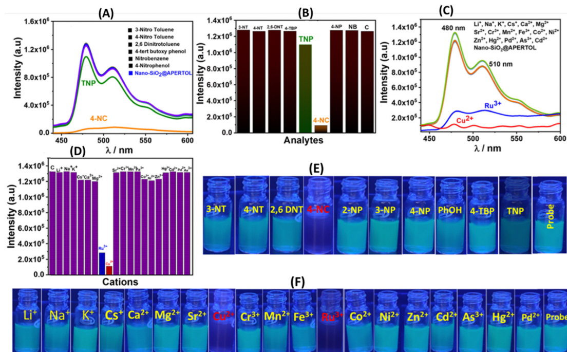
Fig. 5 (A)–(D) The fluorescence selectivity response & relative emission intensity of the material nano-SiO 2 @BAPERTOL in the presence of cations & nitro-analytes; (E) and (F) the selective fluorescence quenching pictures of the material with the specific analytes 4-NC, Cu 2+ and Ru 3+ in the presence of other ions.
