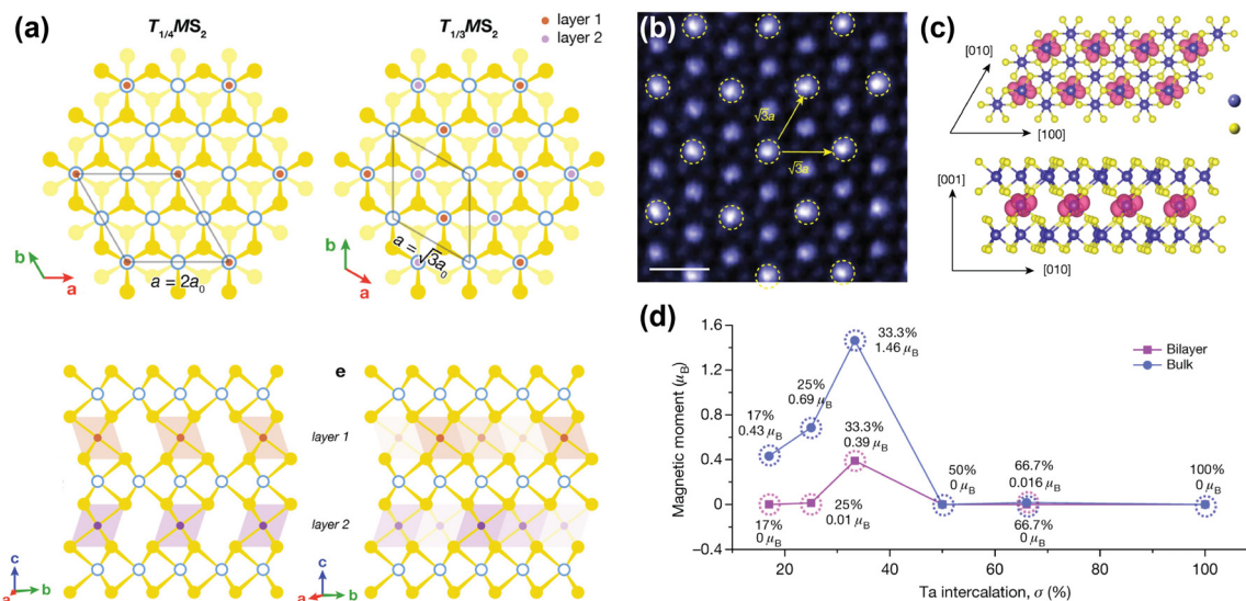
Fig. 4 Inducing magnetic order through transition metal intercalation. (a) Superlattices of \text{Fe}_x\text{MS}_2 and \text{Cr}_x\text{MS}_2 with \text{M} = \text{Nb} or \text{Ta} , for x = 1/4 and x = 1/3 . 144 (b) Atomic-resolution STEM-ADF (scanning transmission electron microscopy – angular dark field) image of self-intercalated \text{Ta}_7\text{S}_{12} , showing the superstructure of the intercalated Ta ions. The scale bar corresponds to 0.5 nm. 152 (c) Top view (top) and side view (bottom) of the spin density isosurface of the intercalated Ta in \text{Ta}_7\text{S}_{12} . 152 (d) Calculated magnetic moments as a function of Ta intercalation ( \sigma ) in \text{TaS}_2 . 152 Reprinted with permission from ref. 144. Copyright 2022 American Chemical Society. Reproduced from ref. 152 with permission from Springer Nature, copyright 2020.
