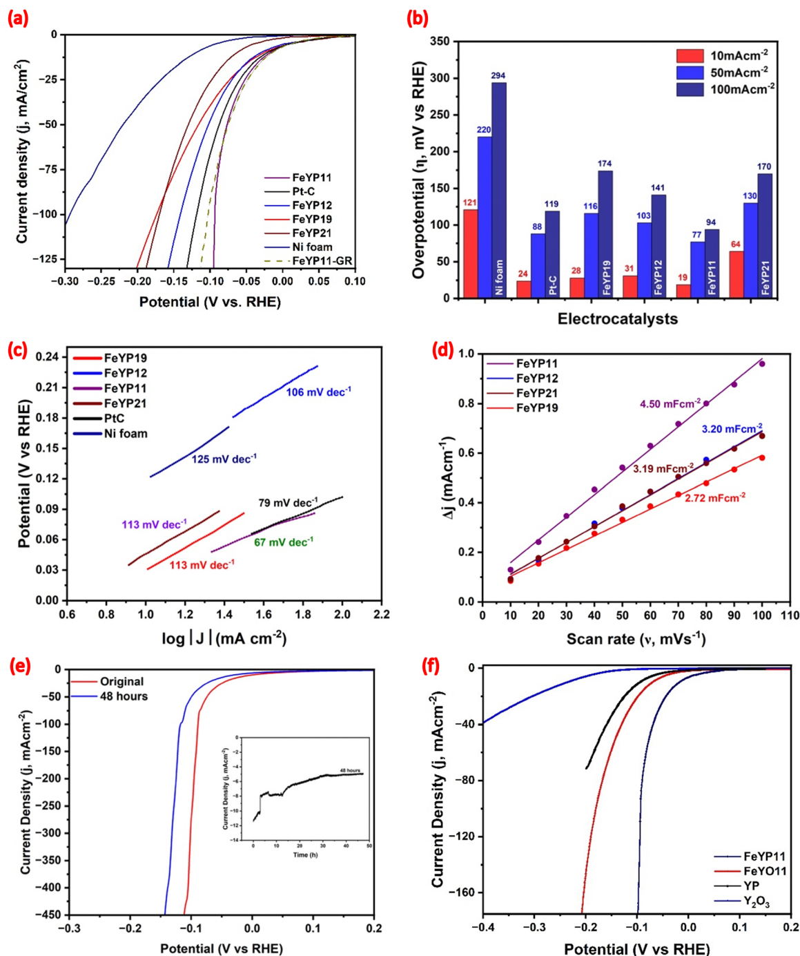
Fig. 5 HER performance of the as-prepared samples. (a) Polarization curves at a 10 \text{mV s}^{-1} scan rate, (b) comparative bar diagrams of overpotential at different current densities, (c) Tafel plots, (d) double-layer capacitance measurements, (e) the chronopotentiometry curve of FeYP11, and (f) polarization curves of FeYP11, FeYO11, YP and \text{Y}_2\text{O}_3 in 1 M KOH solution.
