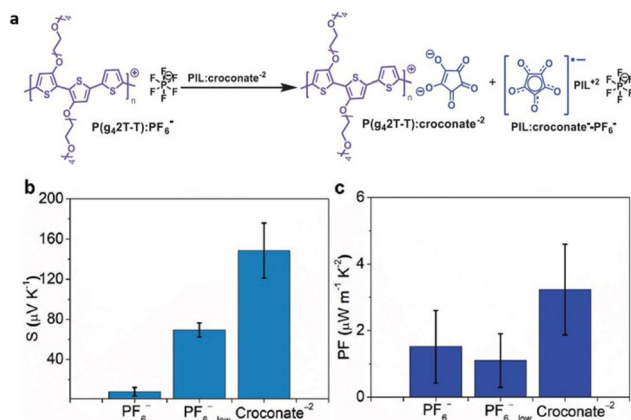
Fig. 54 (a) Structure of the P(g_42T-T) with croconate^{2-} . Thermoelectric parameters of chemically doped and ion exchange P(g_42T-T) films. (b) Seebeck coefficients ( S ) and (c) power factors ( PF ) of P(g_42T-T):PF_6^- , P(g_42T-T):PF_6^- low, and P(g_42T-T):croconate^{2-} thin films. Reproduced from ref. 234 with permission from Wiley-VCH, Copyright [2023].
