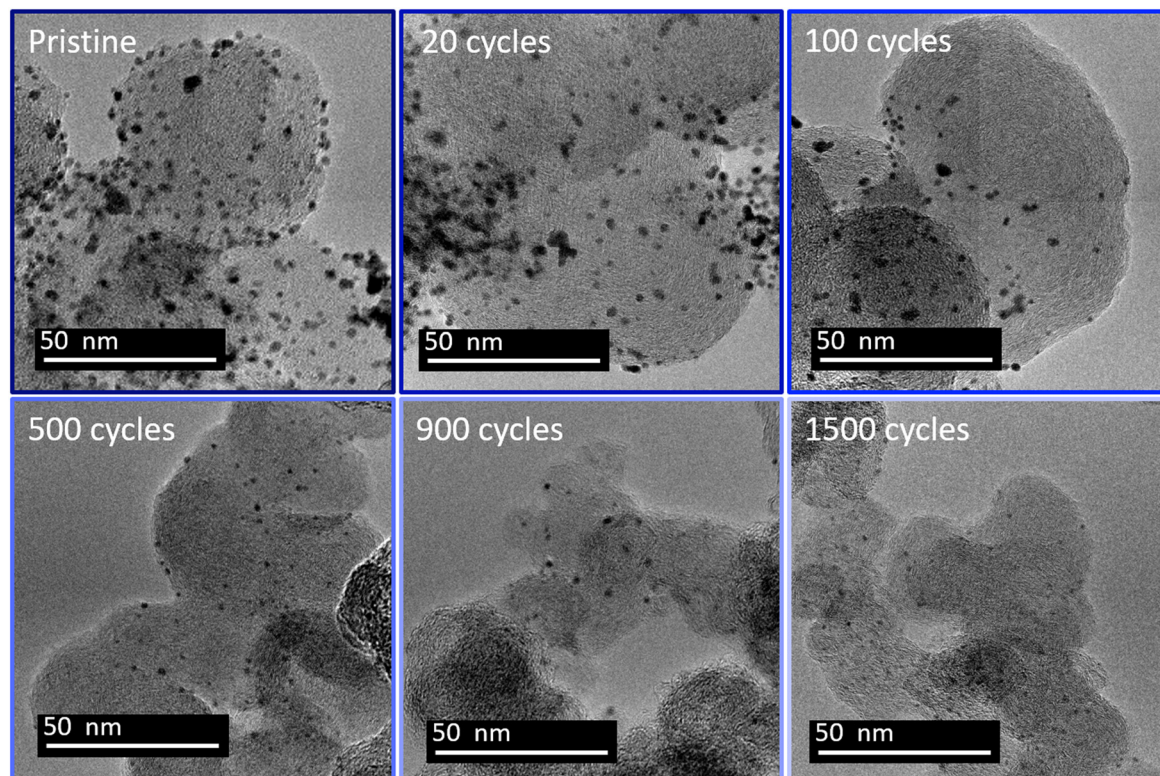
Fig. 3 Representative TEM images of platinum particles from a Pt/C 20% TKK at 20 \mu\text{g cm}^{-2} loading at different stages of cycling between 1.2 and 0.85 V vs. RHE in 1 M \text{H}_2\text{SO}_4 + 0.01 M NaCl.
