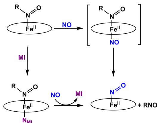
Scheme 3 Summary of the reactivity observed for five- and six-coordinate ferrous heme-RNO ( \text{R} = \text{IPr} and \text{PhNO} ) complexes with the \text{TPP}^{2-} ligand with NO.
