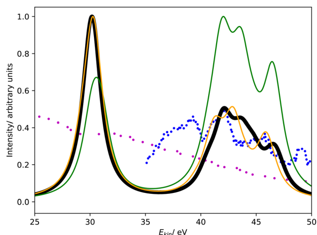
Fig. 3 \text{L}_1\text{L}_{2,3}\text{M} Coster–Kronig spectrum of hydrogen sulfide. Partial decay widths were computed with CBF-EOM-CCSD (black solid line), Fano-EOM-CCSD (orange solid line), and assuming the same width for every channel (green solid line). The experimental data reported in ref. 47 and 46 are shown as blue and purple dotted lines. The theoretical spectra are shifted to higher kinetic energy by 7.5 eV.
