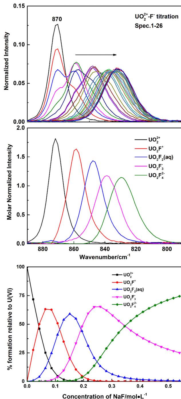
Fig. 1 Representative Raman spectral titration of \text{U(VI)} with fluoride. Top: Spectra collected during a titration (normalized to the intensity of 0.257 M perchlorate). Middle: Raman spectra of \text{U(VI)} /fluoride complexes of relative intensity from deconvolution. C_{\text{uranyl}} = 0.074\text{ M} , C_{\text{perchlorate}} = 0.257\text{ M} , V = 0.66\text{ mL} , C_{\text{H}^+} = 0.003\text{ M} , C_{\text{fluoride}} = 0\text{--}0.54\text{ M} . Bottom: Speciation distribution during the titration.
