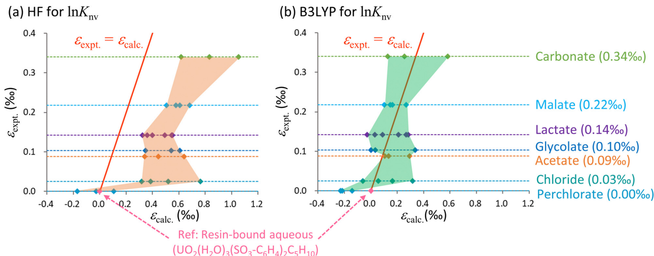
Fig. 3 Calculated \epsilon values based on \ln K_{nv} obtained using the (a) HF and (b) B3LYP methods along with experimental data for the \text{U}(\text{vi}) – \text{U}(\text{vi}) system. The horizontal axis shows the calculated values relative to \text{UO}_2(\text{H}_2\text{O})_3(\text{SO}_3-\text{C}_6\text{H}_4)_2\text{C}_5\text{H}_{10} while the vertical axis shows the experimental values relative to the aqueous \text{UO}_2^{2+} complex bound to the cation exchange resin. The red solid line indicates the scenario in which the calculated and experimental values are equal. The areas bounded by the values calculated using the HF and B3LYP methods are shaded orange and green, respectively. The dotted lines parallel to the horizontal axis represent the experimental values for each species as described on the right while the quantities in parentheses indicate the experimental data. The numerical data are also summarized in Table 3.
