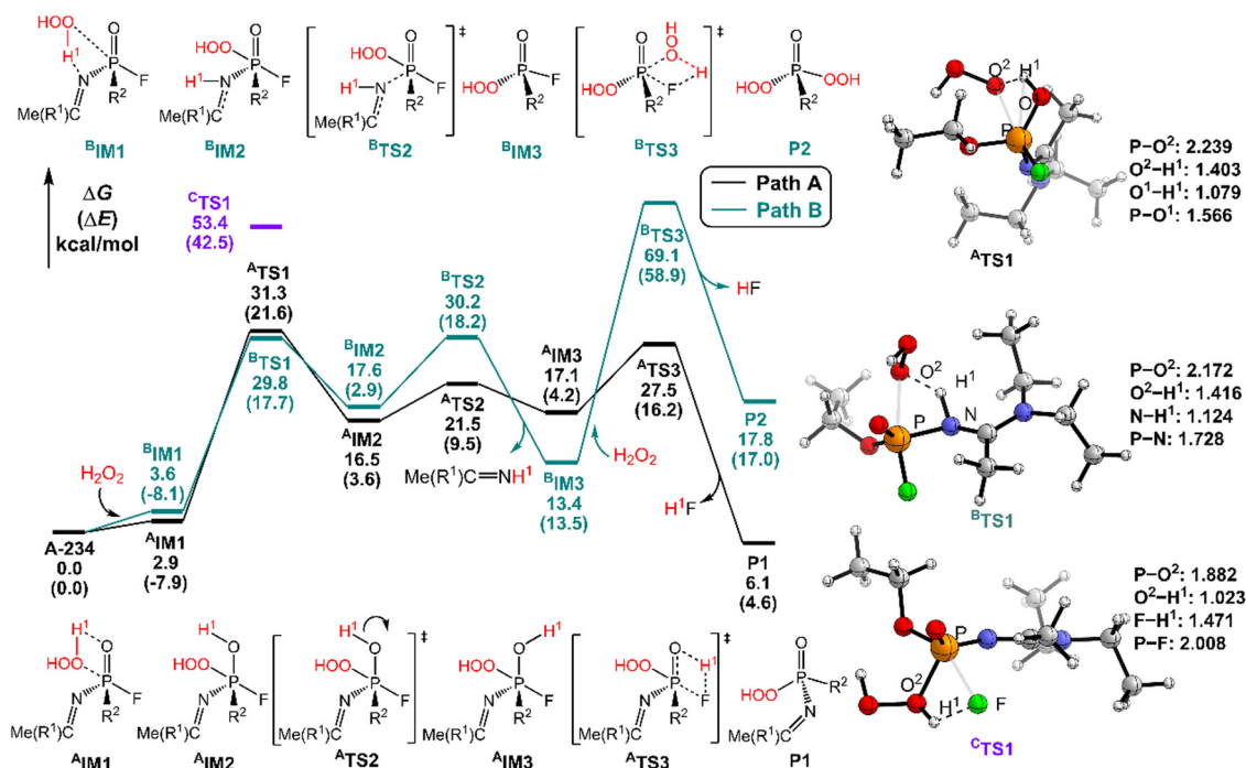
Fig. 2 Predicted relative free energy profiles ( \Delta G in \text{kcal mol}^{-1} ) and electronic energies ( \Delta E in parentheses) of the species involved in the perhydrolysis of A-234 by \text{H}_2\text{O}_2 . The main transition state structures and the selected key bond lengths (in Å) are given.
