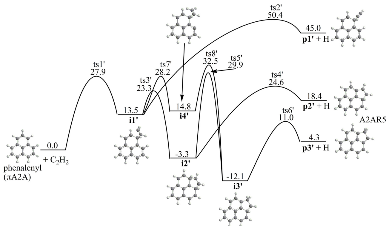
Fig. 1 Potential energy diagram for the \text{C}_{13}\text{H}_9 (phenalenyl, \pi\text{A2A} ) + \text{C}_2\text{H}_2 reaction. All relative energies given in kcal mol -1 with respect to the initial reactants are calculated at the G3(MP2,CC)//B3LYP/6-311G(d,p)+ZPE(B3LYP/6-311G(d,p)) level of theory.
