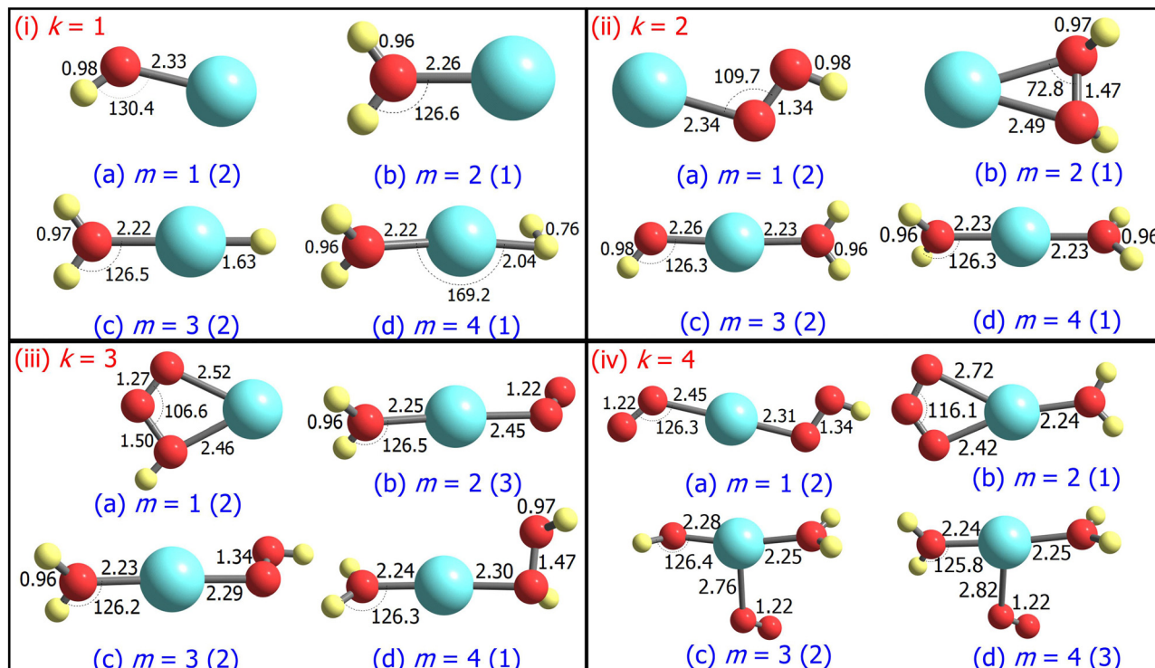
Fig. 1 Ground state structures of \text{AgO}_k\text{H}_m^+ , where k, m = 1-4 , optimized at the CCSD level. Bond lengths and angles are given in Å and degrees, respectively. The spin multiplicity ( 2S + 1 ) of the \text{AgO}_k\text{H}_m^+ clusters is provided in the parentheses.
