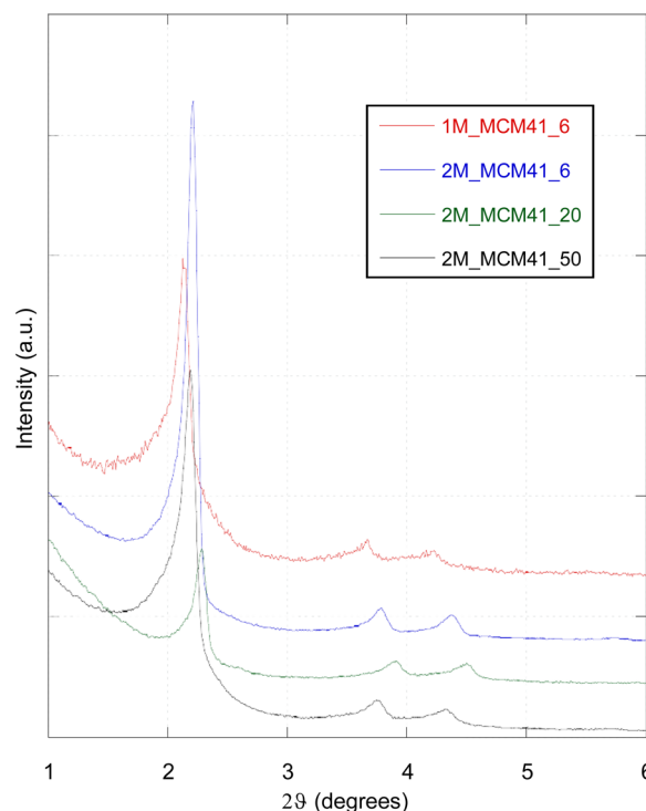
Fig. 5 Low-angle X-ray powder diffraction patterns of the magnetic MCM41-like materials (M_MCM41 samples).
