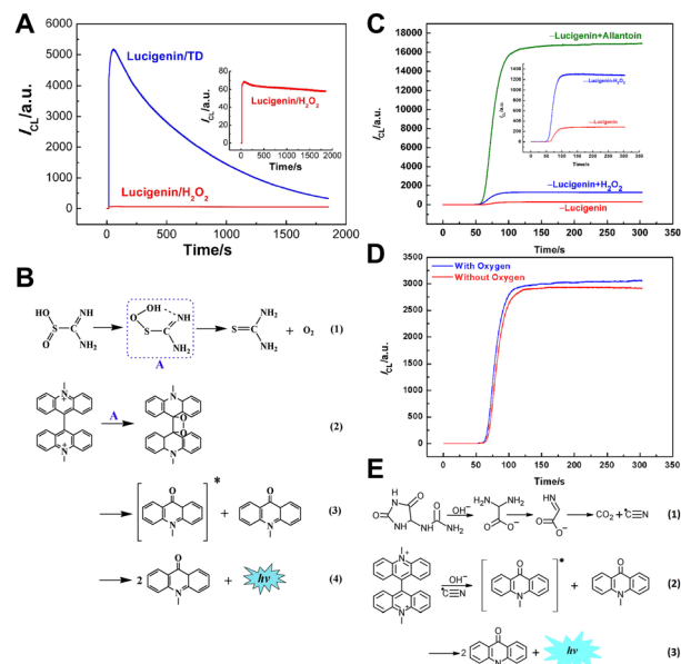
Fig. 4 (A) The CL intensity–time curves of the lucigenin/H 2 O 2 and lucigenin/TD systems. Inset: enlarged CL intensity–time curve of the lucigenin/H 2 O 2 system. [lucigenin]: 10.0 μM; [TD]: 1.0 mM; [H 2 O 2 ]: 1.0 mM; [NaOH]: 0.5 M; PMT voltage: −700 V. (B) Reaction mechanism of the lucigenin/TD CL system. Reprinted with permission from ref. 43, Copyright 2016 Elsevier. (C) CL intensity–time curves of the lucigenin/H 2 O 2 and lucigenin/allantoin systems. The inset focuses on the enlarged CL intensity/time curve of lucigenin and lucigenin/H 2 O 2 systems. 1.5 M NaOH, 0.1 mM lucigenin, 2 mM H 2 O 2 , and 2 mM allantoin. PMT voltage: −800 V. (D) CL kinetic profiles in the presence and absence of oxygen. 1.5 M NaOH, 0.1 mM lucigenin and 2 mM allantoin. PMT voltage: −600 V. (E) Possible mechanism of the lucigenin/allantoin CL system. Reprinted with permission from ref. 44, Copyright 2017 American Chemical Society.
