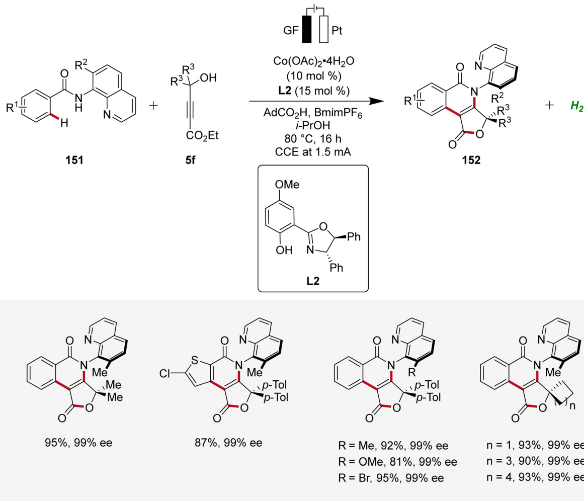
Scheme 48 Atroposelective cobaltalelectro-catalyzed C–H alkyne cascade annulation.
