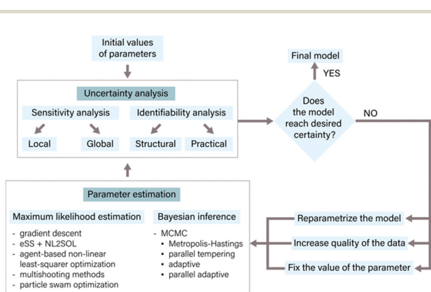
Fig. 3 The main steps of parameter estimation. The estimation process is iterative and continues until the desired level of certainty is achieved. It begins with an initial guess of parameter values derived from literature or expert knowledge, followed by uncertainty analysis that quantifies the uncertainty in the model parameters and its impact on predictions. The results of uncertainty analysis guide reparameterization and potential data generation. Various parameter estimation methods such as maximum likelihood estimation, Bayesian inference, or evolutionary algorithms can be employed. Another round of uncertainty analysis evaluates the uncertainty in newly estimated parameters. This iterative process enhances the reliability and accuracy of the evolutionary model's predictions.
