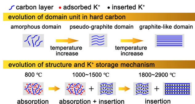
Fig. 2 Illustration of hard carbon with different microstructures (above) and its corresponding K^+ storage mechanism (below). (Reprinted with permission from ref. 56. Copyright 2022 American Chemical Society).
