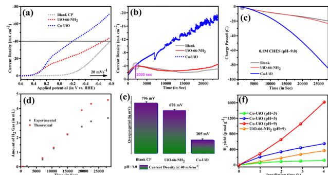
Fig. 2 (a) Comparative linear sweep voltammetry (LSV) data recorded for the catalyst-modified electrodes at pH \sim 9.0 . LSV was recorded after CV stabilised at 20 \text{ mV s}^{-1} scan rate; data were recorded at room temperature using 0.1 \text{ M} CHES buffer. The active surface area of the CP-modified electrode was 0.25 \text{ cm}^2 . (b) Chronoamperometric current passed with time during the fixed potential electrolysis at -0.490 \text{ V} in a 0.1 \text{ M} CHES buffer (pH \sim 9.0 ) (the purple circle indicated the boost in HER activity). (c) Chronocoulometric charge passed during the fixed potential electrolysis at -0.472 \text{ V} (the purple circle indicated the boost in HER activity). [In Figure a, b, c; Gray trace: blank CP, red trace: UiO-66-NH 2 modified CP, and blue trace: Co-UiO modified CP.] (d) The experimentally (black trace) and theoretically (red trace) measured volume of H 2 gas during the bulk electrolysis at pH \sim 9.0 . (e) Comparative bar diagram for the overpotential requirement to attain 40 \text{ mA cm}^{-2} current density during the LSV experiment performed at pH \sim 9.0 ; and (f) time course of the photocatalytic H 2 production curves.
