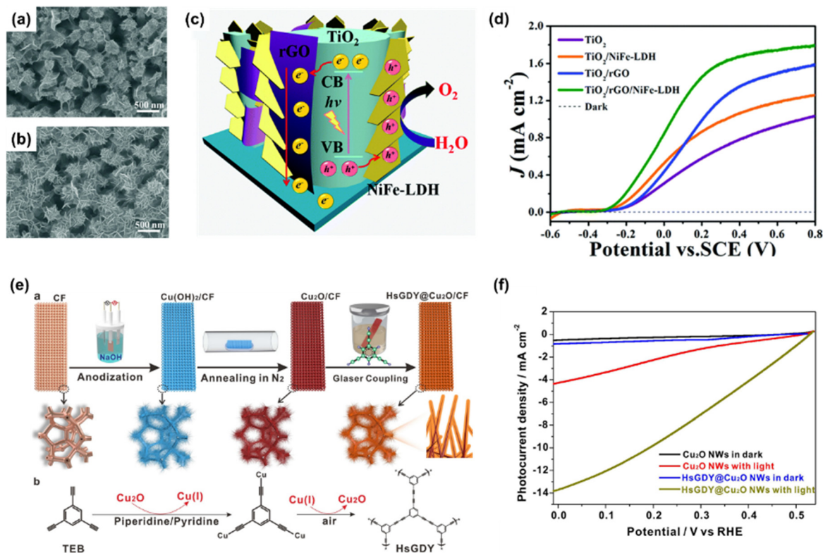
Fig. 7 SEM images of (a) \text{TiO}_2/\text{NiFe-LDH} NAAs and (b) \text{TiO}_2/\text{rGO}/\text{NiFe-LDH} NAAs. (c) Schematic of the PEC water oxidation process in the \text{TiO}_2/\text{rGO}/\text{NiFe-LDH} core-shell NA photoanode. (d) LSV curves of \text{TiO}_2 , \text{TiO}_2/\text{NiFe-LDH} , \text{TiO}_2/\text{rGO} , and \text{TiO}_2/\text{rGO}/\text{NiFe-LDH} NAAs. Copyright 2016, Royal Society of Chemistry. (e) Schematic illustration of the fabrication of \text{HsGDY}@/\text{Cu}_2\text{O}/\text{CF} photocathode. (f) LSV curves of \text{Cu}_2\text{O} NWs and \text{HsGDY}@/\text{Cu}_2\text{O} NWs. Copyright 2022, Springer Nature.
