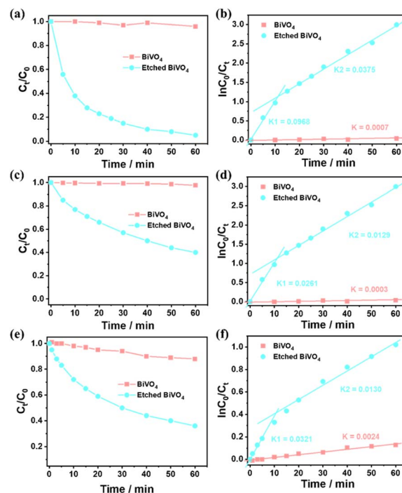
Fig. 5 (a) Photocatalytic degradation of methyl blue over a decahedron \text{BiVO}_4 crystal and etched \text{BiVO}_4 crystal. (b) Corresponding rate constants of methyl blue degradation from (a). (c) Photocatalytic degradation of methyl orange over a decahedron \text{BiVO}_4 crystal and etched \text{BiVO}_4 crystal. (d) Corresponding rate constants of methyl orange degradation from (c). (e) Photocatalytic degradation of m -cresol over a decahedron \text{BiVO}_4 crystal and etched \text{BiVO}_4 crystal. (f) Corresponding rate constants of m -cresol degradation from (e). Reaction conditions: catalyst, 200 mg; 10.0 \text{mg L}^{-1} organic molecules, 100 mL; light source, Xe lamp (300 W). The etched \text{BiVO}_4 crystal represents a \text{BiVO}_4 crystal treated in 2.0 M NaOH solution for 2.5 h.
