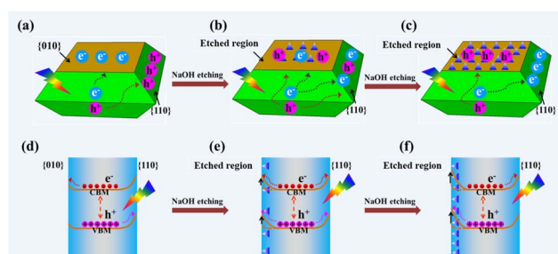
Fig. 4 Scheme of the distribution of photogenerated electrons and holes on a decahedron \text{BiVO}_4 crystal (a) before and (b and c) after NaOH etching. Scheme of different band bendings in the etched region and \{110\} facets of the decahedron \text{BiVO}_4 crystal (d) before and (e and f) after NaOH etching and the resulting spatial charge separation.
